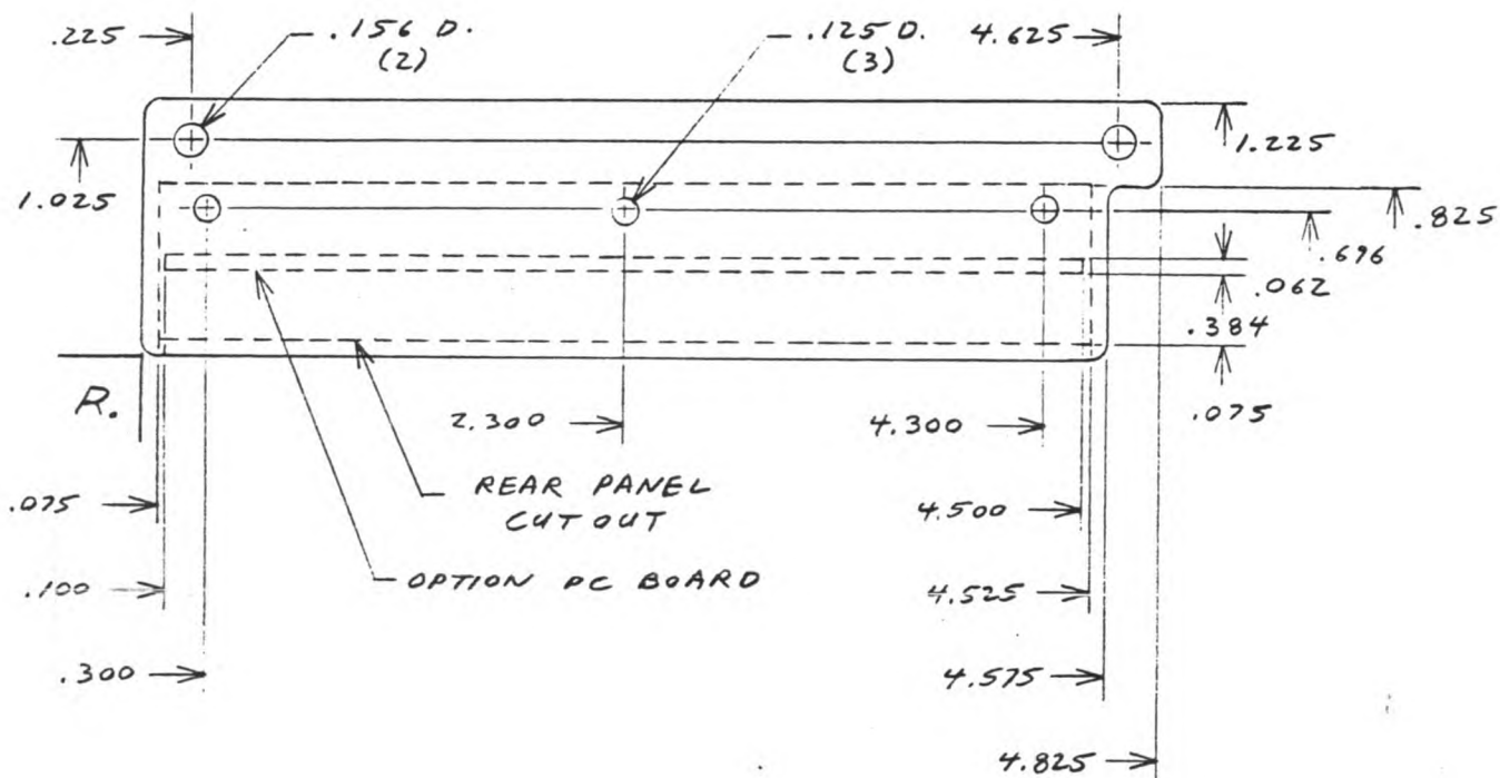
FIGURE 4 - OPTION REAR PANEL (.050 ALUMINUM)
