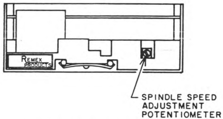
REAR VIEW OF A REMEX DISK DRIVE SHOWING LOCATION OF THE SPEED ADJUSTMENT POTENTIOMETER
