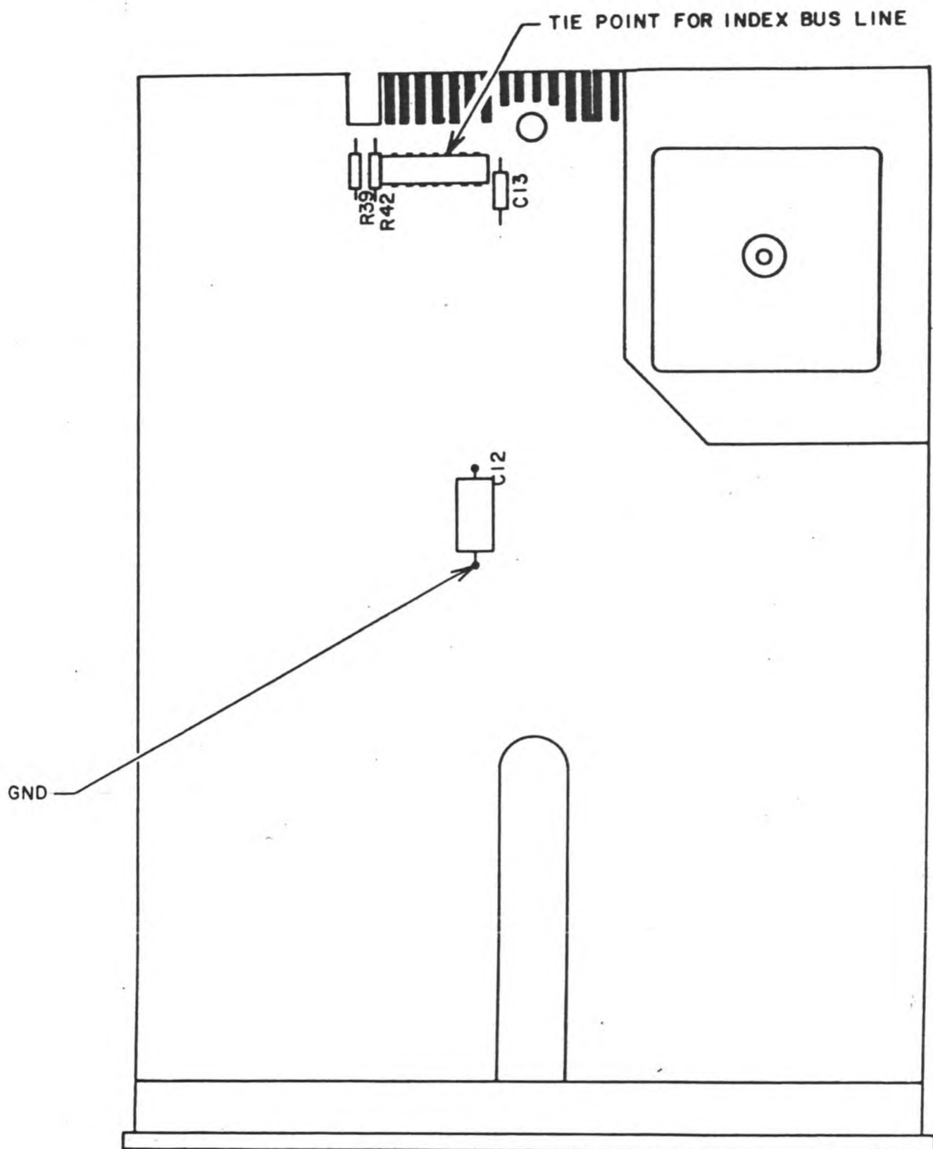
TOP VIEW OF A REMEX DISK DRIVE SHOWING TIE POINT FOR USING A FREQUENCY COUNTER TO ADJUST SPINDLE SPEED
