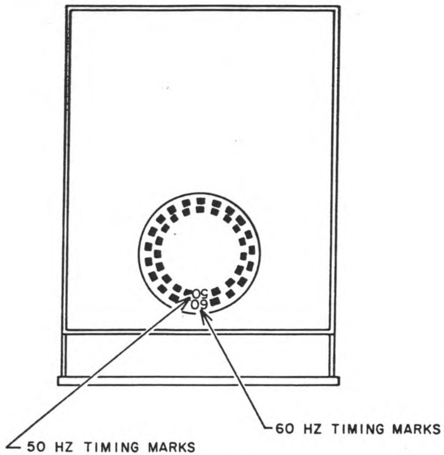
BOTTOM VIEW OF A REMEX DISK DRIVE SHOWING TIMING MARKS
