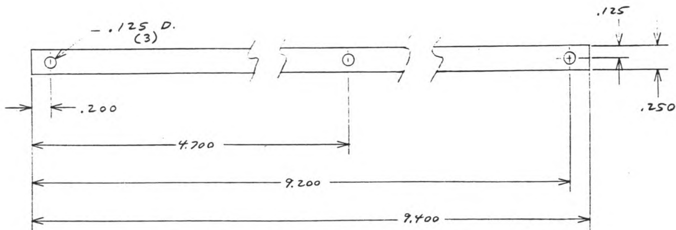
FIGURE 3 - STIFFENER (.031 ALUMINUM)
